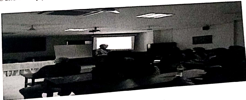
Figure 1 Mathematics_NET_GATE
