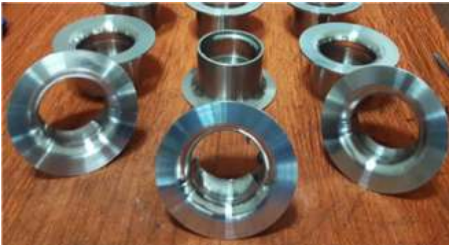
Connecting Flange HAL(MIG-21)
